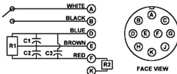
Wiring Diagram C870-1025 Foot Control
