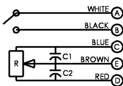
WIRING DIAGRAM C810-1425 AND C810-0525 TIG WELDING FOOT CONTROLS
