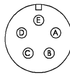
PLUG FACE VIEW C810-0525
