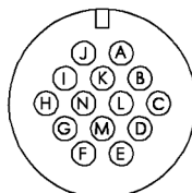
PLUG FACE VIEW C810-1425
