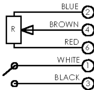
Wiring Diagram C860-0625 Foot Control
